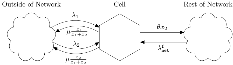
FIGURE 1. Description of the model considered in the paper. Without imposing the balance condition corresponding to the fixed-point equation (FP), this is a two-class Processor-Sharing queue with one impatient class, namely the class-2 of mobile users, with arrival rate \lambda_2 + \lambda_{\text{net}}^f = \lambda_{\text{tot}}^f . The balance equation (FP) accounts for the fact that a typical cell at equilibrium is considered, with equal flows from and to the rest of the network.
